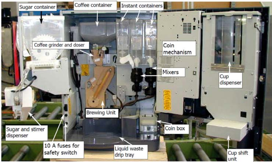
BRIO 250: VIEW WITH DOOR OPEN
